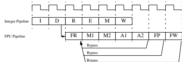
Figure 3 FPU Pipeline
