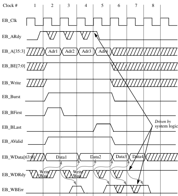
Figure 14 Burst Write Transaction Timing Diagram
